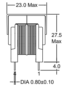
Orthographic view
