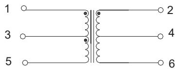
FAT10606S,FAT10609D
