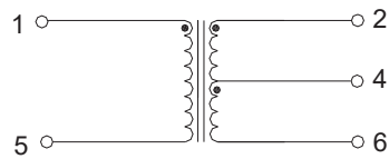
FAT10606D,FAT10608D
