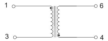
FAT10607D
