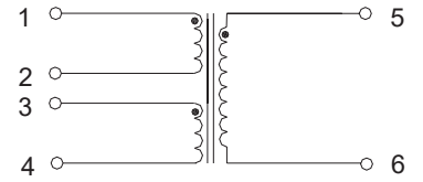
FAT10602S,FAT10605D
